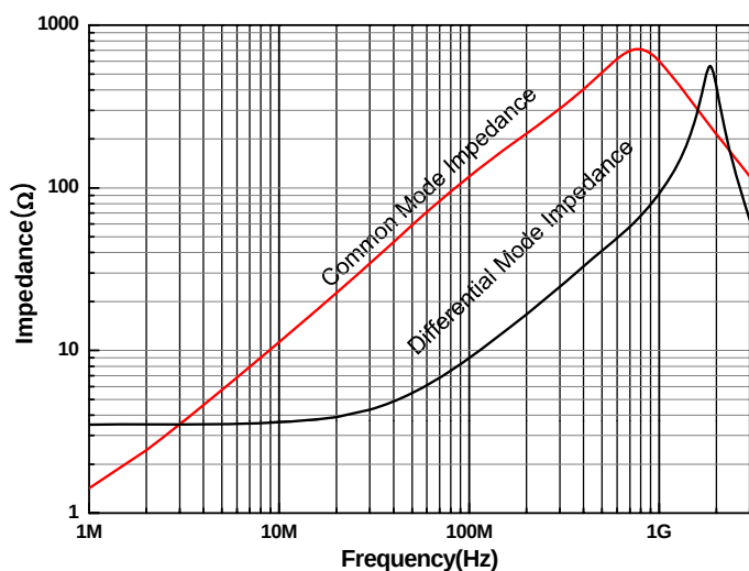
- Impedance Curves
